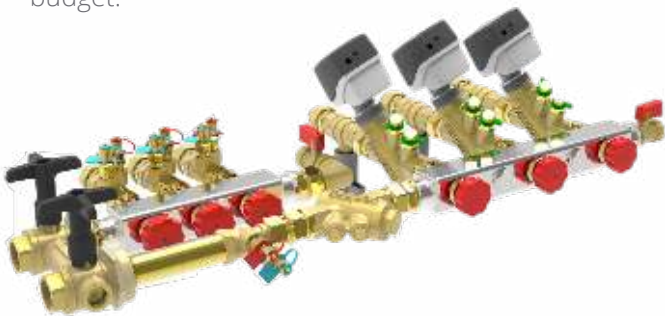
MANIFOLD
